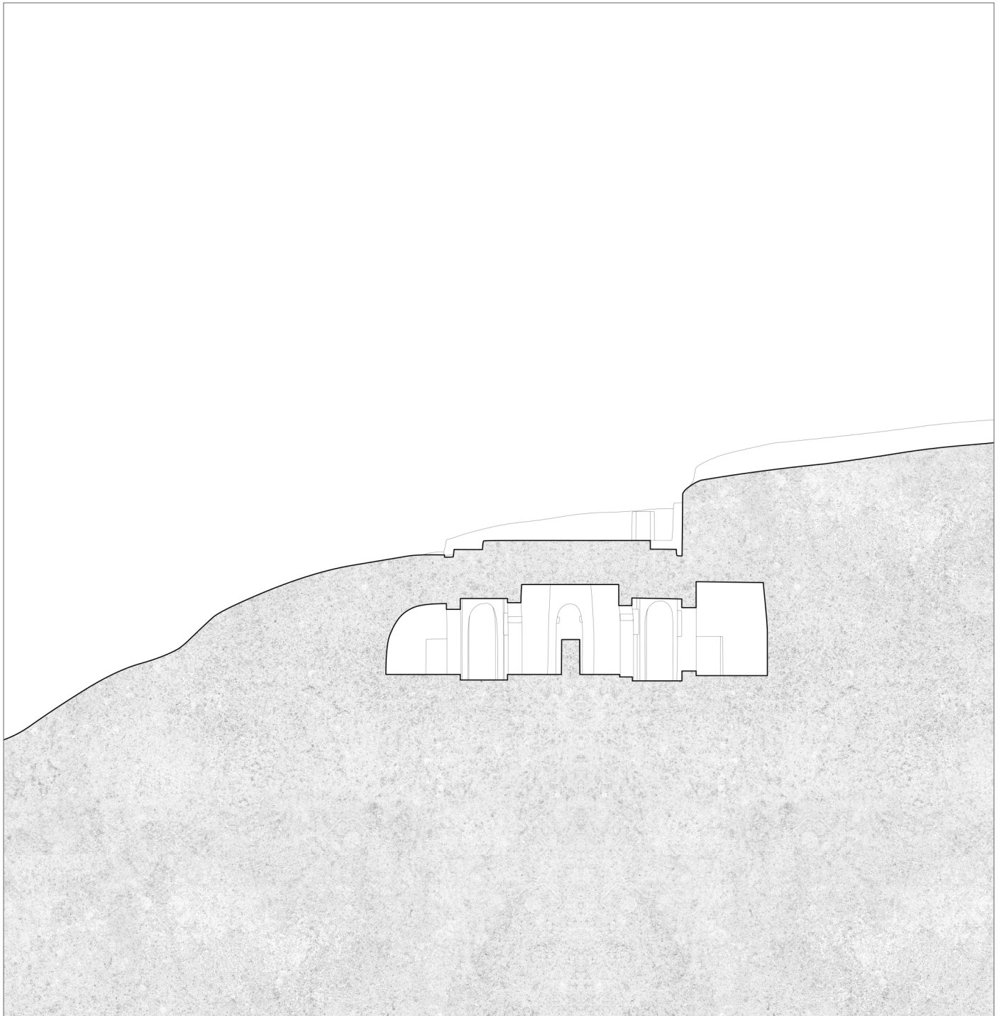
Dagmawi Lalibela (Ambager Complex) Section NN (2015)
